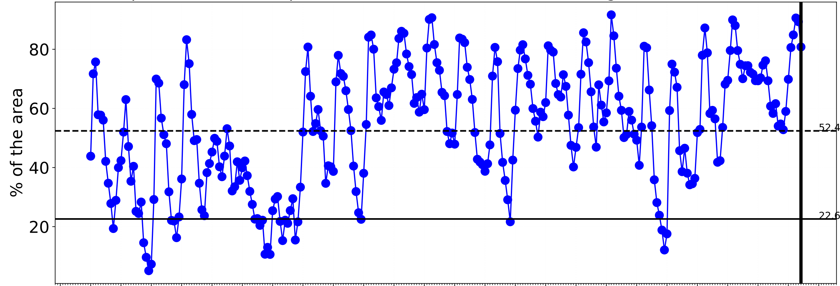
Proportion of the area protected from water erosion (Total Vegetation Cover > 80%)
