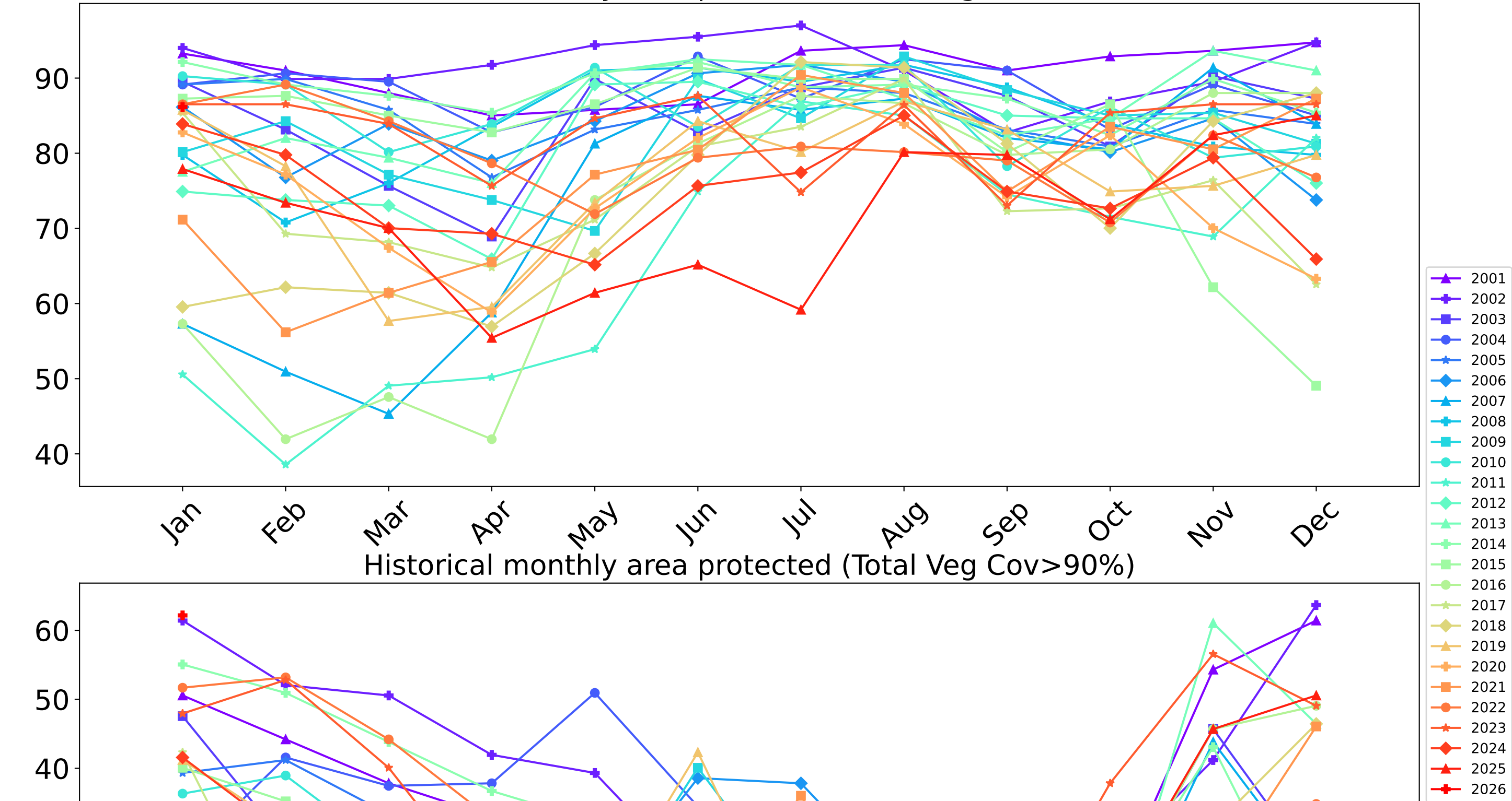
Historical monthly area protected (Total Veg Cov>80%)
