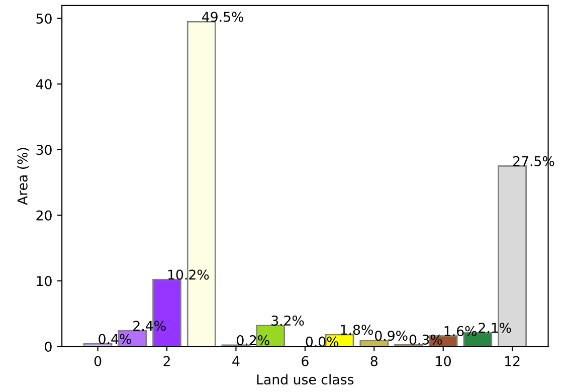
Proportion of each land class in area
