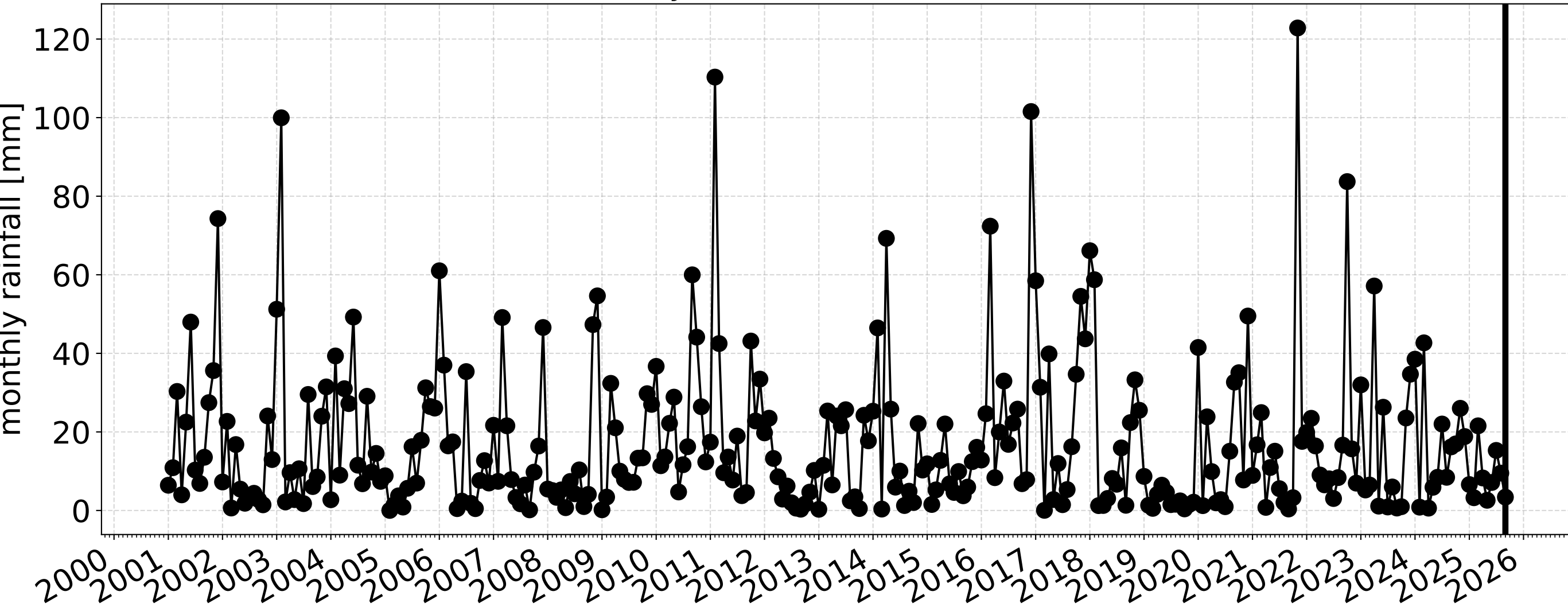
Monthly rainfall from 2001 to 2025
