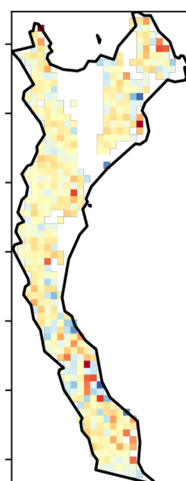
Total Vegetation Cover Anomaly [%]
