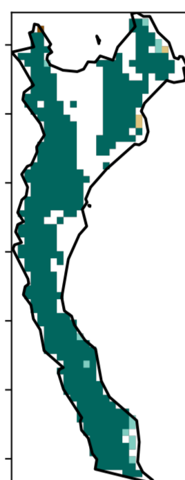
Total Vegetation Cover [%]
