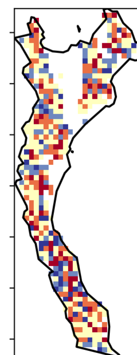
Total Vegetation Cover Decile [%]
