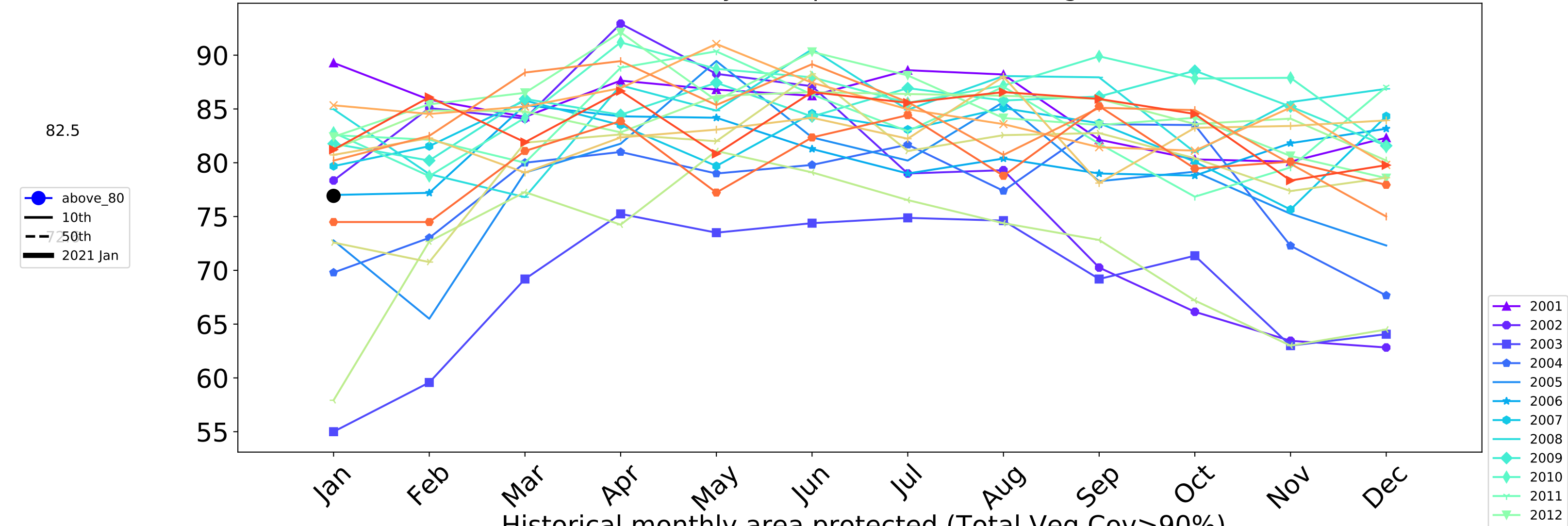
Historical monthly area protected (Total Veg Cov>90%)
