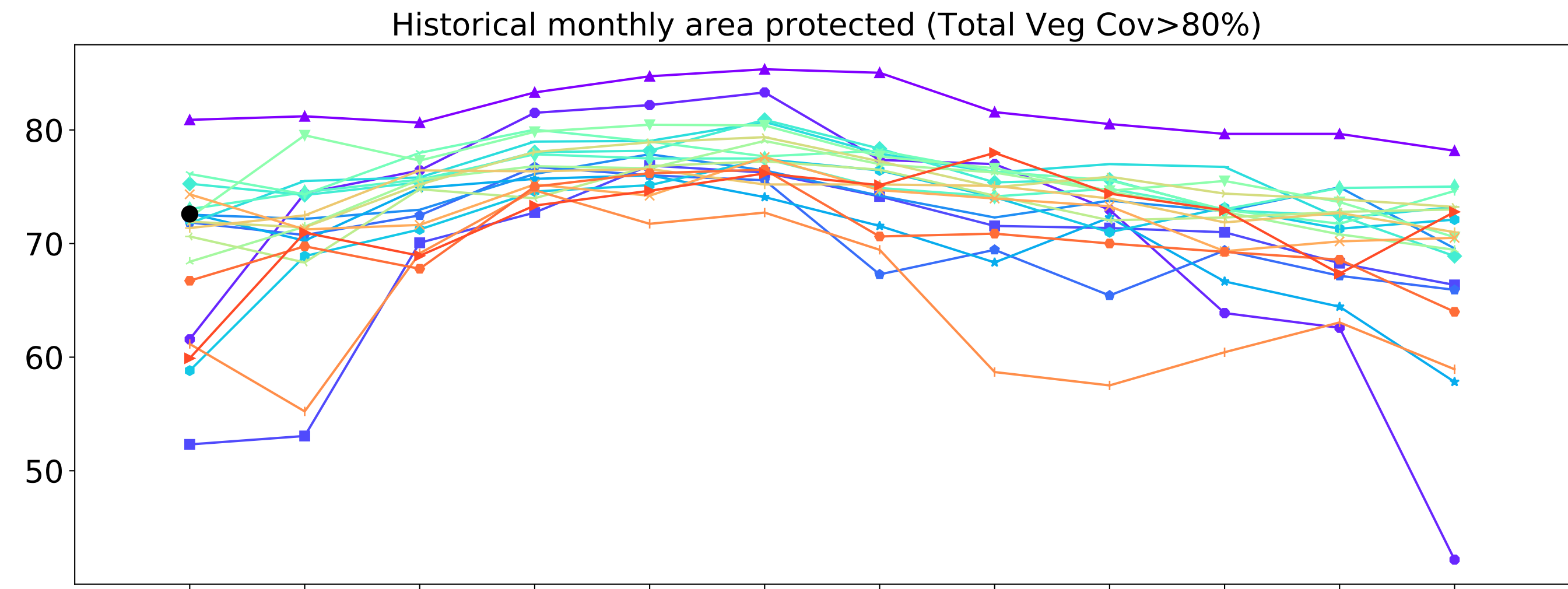
Historical monthly area protected (Total Veg Cov>80%)
