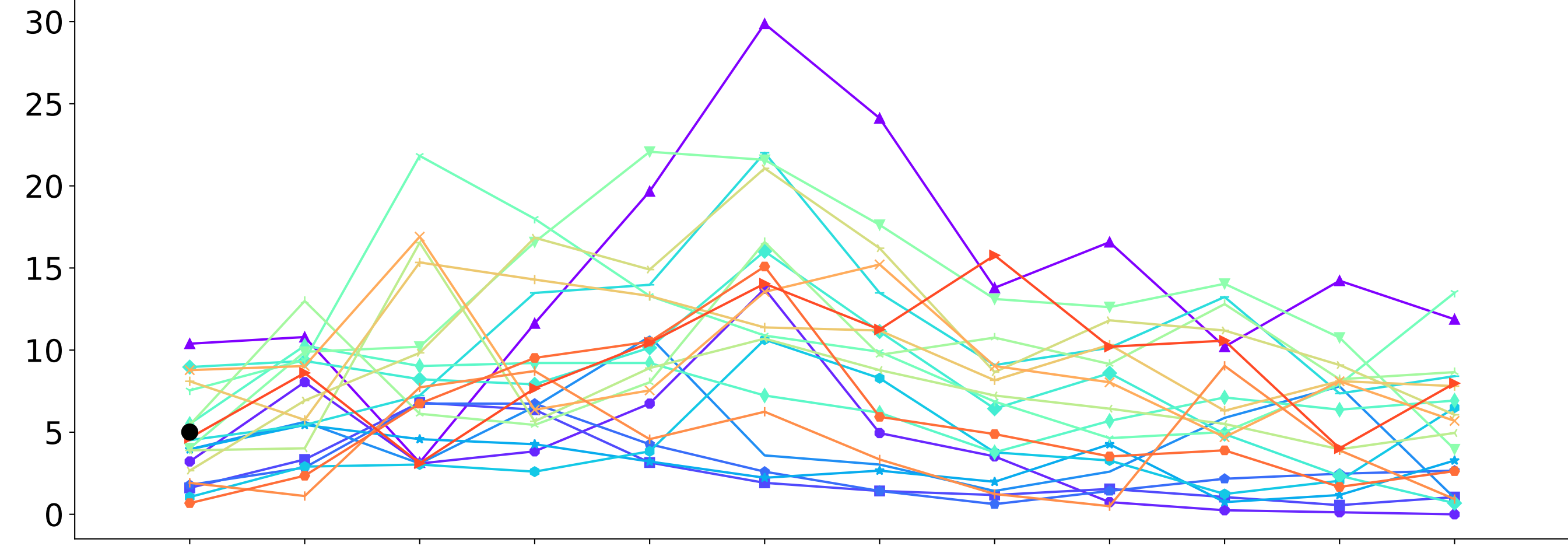
Historical monthly area protected (Total Veg Cov>95%)
