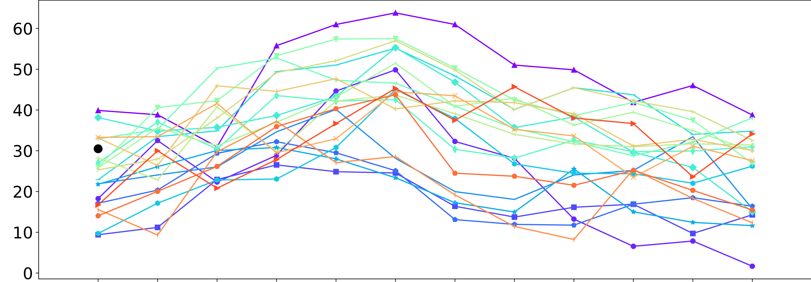
Historical monthly area protected (Total Veg Cov>90%)
